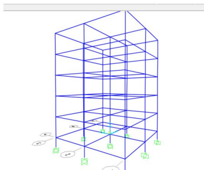
Fig: Showing all members after redesign
