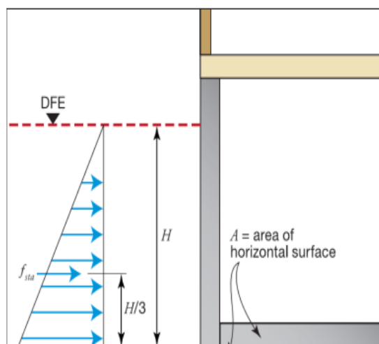
Fig: Hydrostatic load on building
