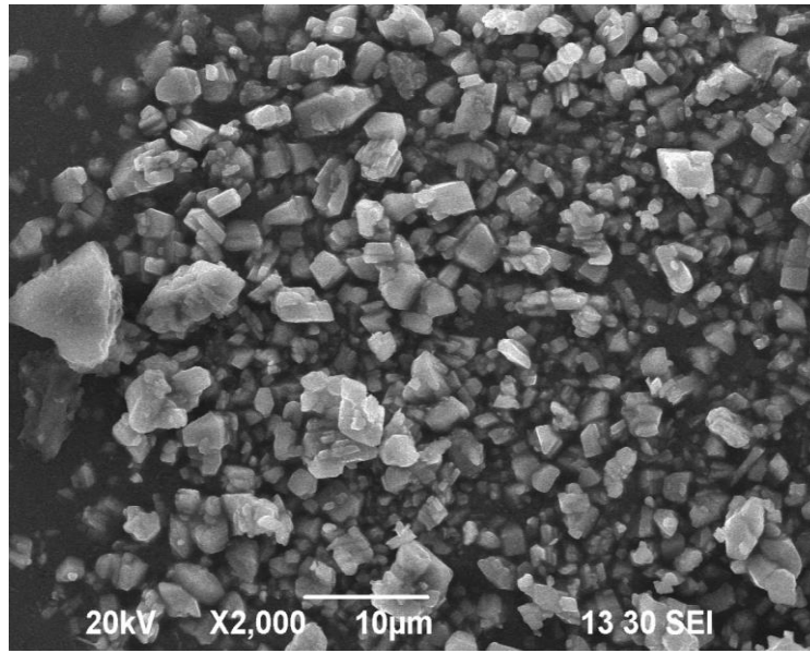
Figure. 3.2a. HR-SEM images of: Prepared ZnO nancomposite material (10 µm)
