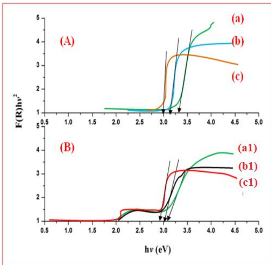
Figure. 3.3. UV-Vis DRS Band gap energy: (A) [(a) ZnO-250 0 C, (b) ZnO-500 0 C, (c) ZnO-600 0 C] and (B) [(a1) Se-ZnO-250 0 C, (b1) Se-ZnO-500 0 C, (c1) Se-ZnO-600 0 C] nanocomposite material
