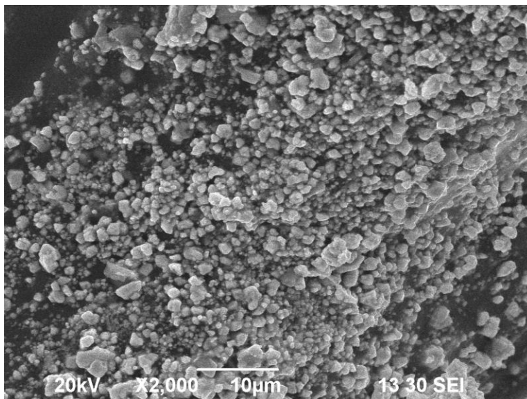
Figure. 3.2b. HR-SEM images of: Prepared Se-doped ZnO nancomposite materials (10 µm)
