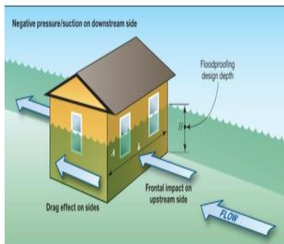
Fig: Hydrodynamic and impact forces
